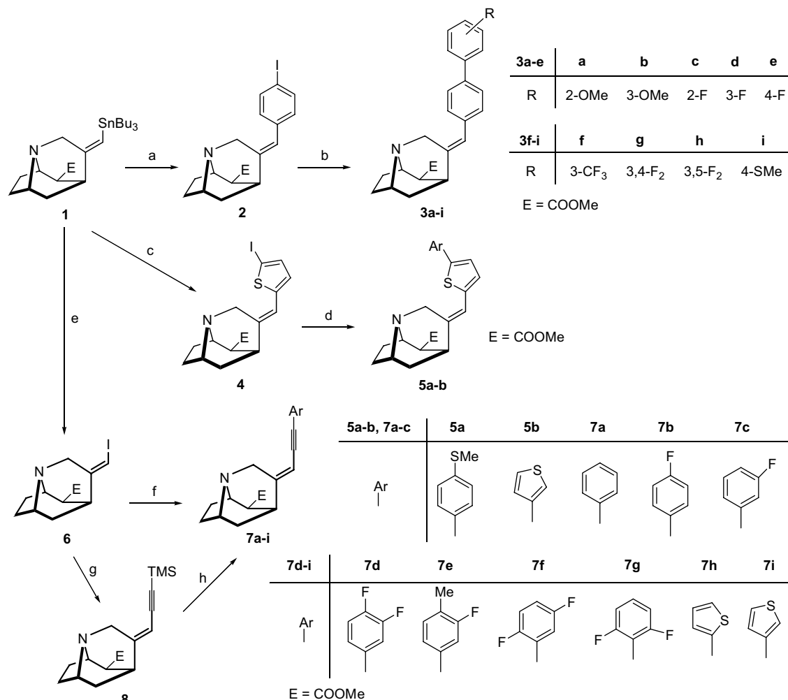
Scheme 1. Synthesis of new conformationally constrained tropanes as NET inhibitors. Reagents and conditions: (a) 1,4-diiodobenzene, Ph 3 As, Pd 2 (dba) 3 , CuI, DMF, 50 °C, 57%; (b) arylboronic acids, Pd(OAc) 2 , K 2 CO 3 , H 2 O/THF, 70–80 °C, 41–78%; (c) 2,5-diiodothiophene, Ph 3 As, Pd 2 (dba) 3 , CuI, DMF, 50 °C, 55%; (d) aryl- or heteroarylboronic acids, Pd(OAc) 2 , K 2 CO 3 , H 2 O/THF, 70–80 °C, 40%; (e) I 2 , CH 2 Cl 2 , rt, 88%; (f) arylacetylenes (for 7a–b and 7i ), PdCl 2 (PPh 3 ) 2 , CuI, Et 3 N, DME, 80 °C, 62–80%; (g) (trimethylsilyl)acetylene, PdCl 2 (PPh 3 ) 2 , CuI, Et 3 N, DME, 80 °C, 17 h, 70%; (h) aryl iodides (for 7c–e and 7h ) or aryl bromides (for 7f–g ), PdCl 2 (PPh 3 ) 2 , CuI, Et 3 N, TBAF, DME, 80 °C, 17–80%.
